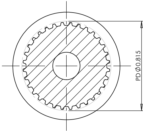
SECTION B-B
